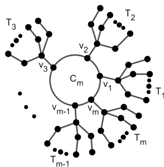
FIGURE 5. Unicyclic graphs U''' .
