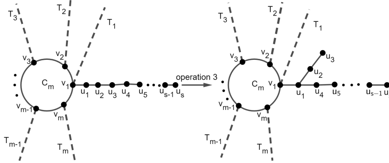
FIGURE 3. Unicyclic graphs U and U' .
