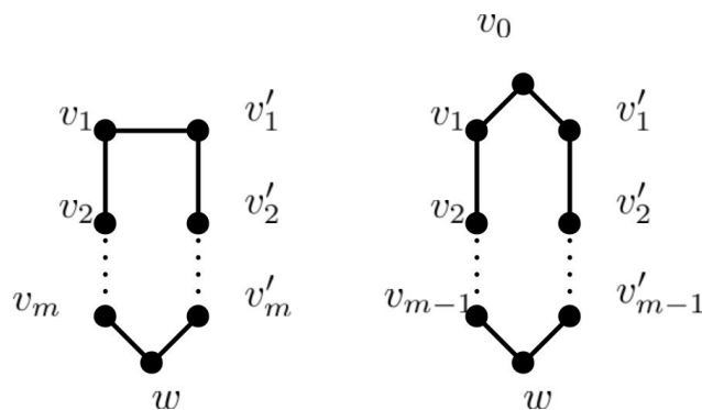
FIGURE 2. The considered polygon (or a cycle of size k ) in the proof of Theorem 2.1.
